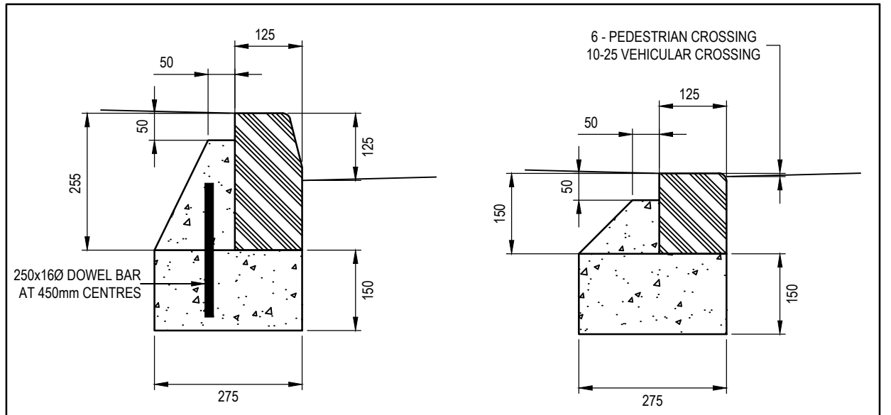
HB2 KERB TYPICAL DETAIL HALF BATTER KERB SCALE 1:10
