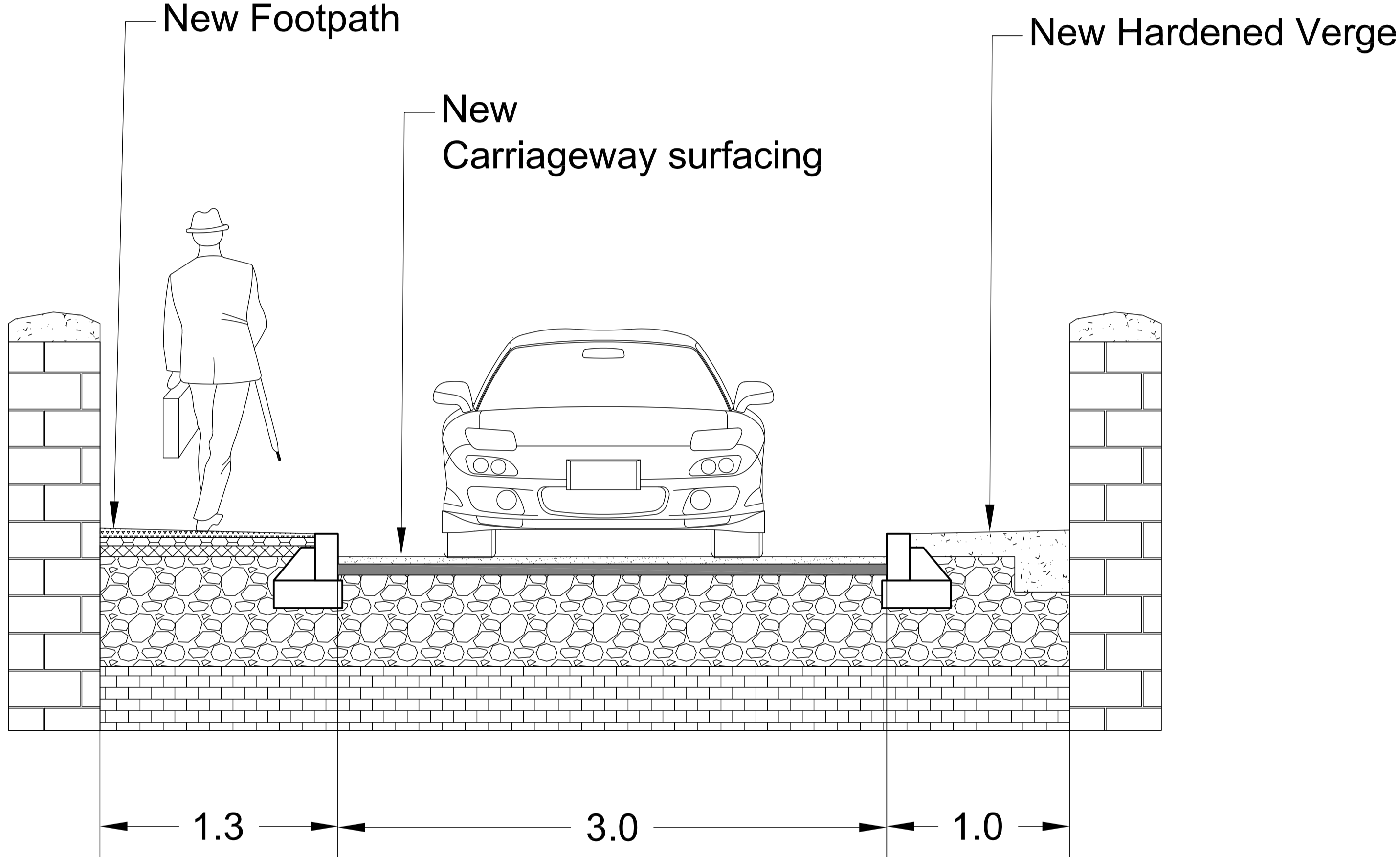
Proposed Cross Section "A-A" of Carriageway & Footway
